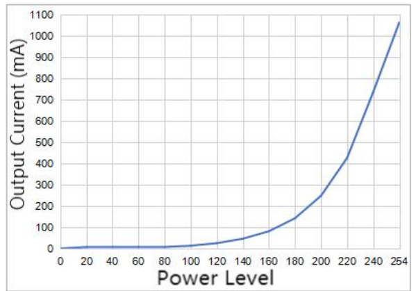
Logarithmic dimming
